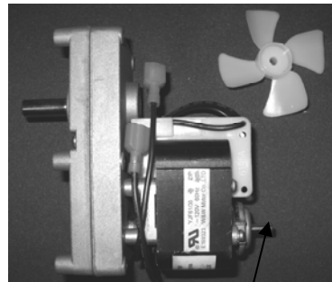
motor shaft
